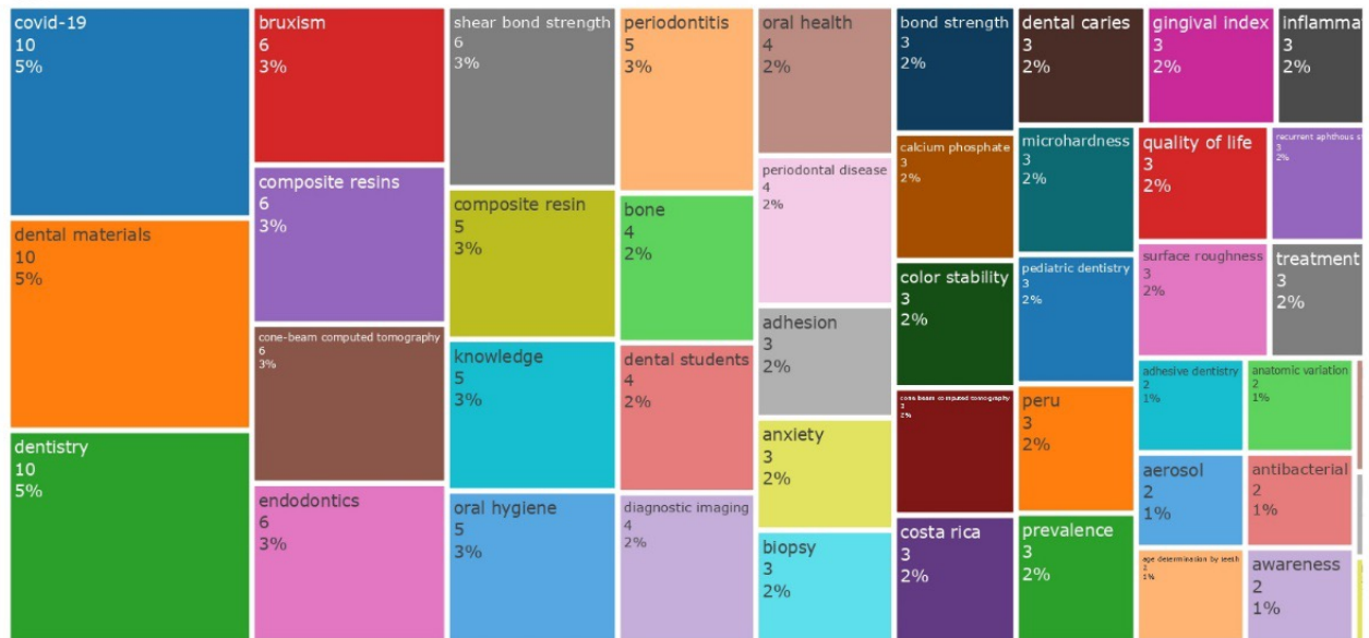
Figure 3. Tree map.
